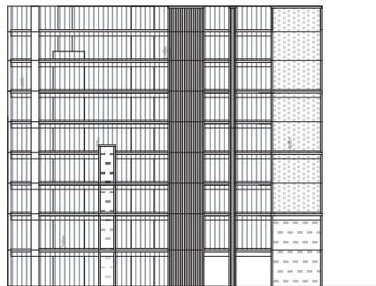
ELEVATION, looking east 1:300
