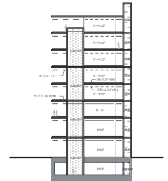
SECTION, B-B 1:300
