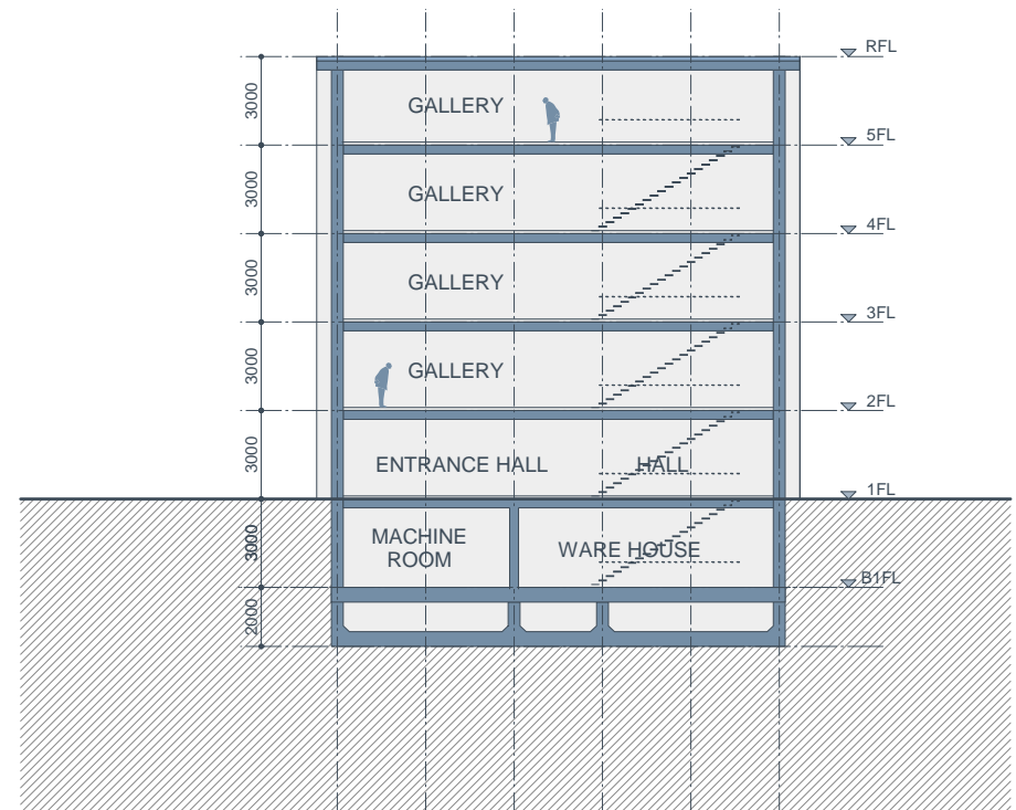
SECTION B-B 1/200
