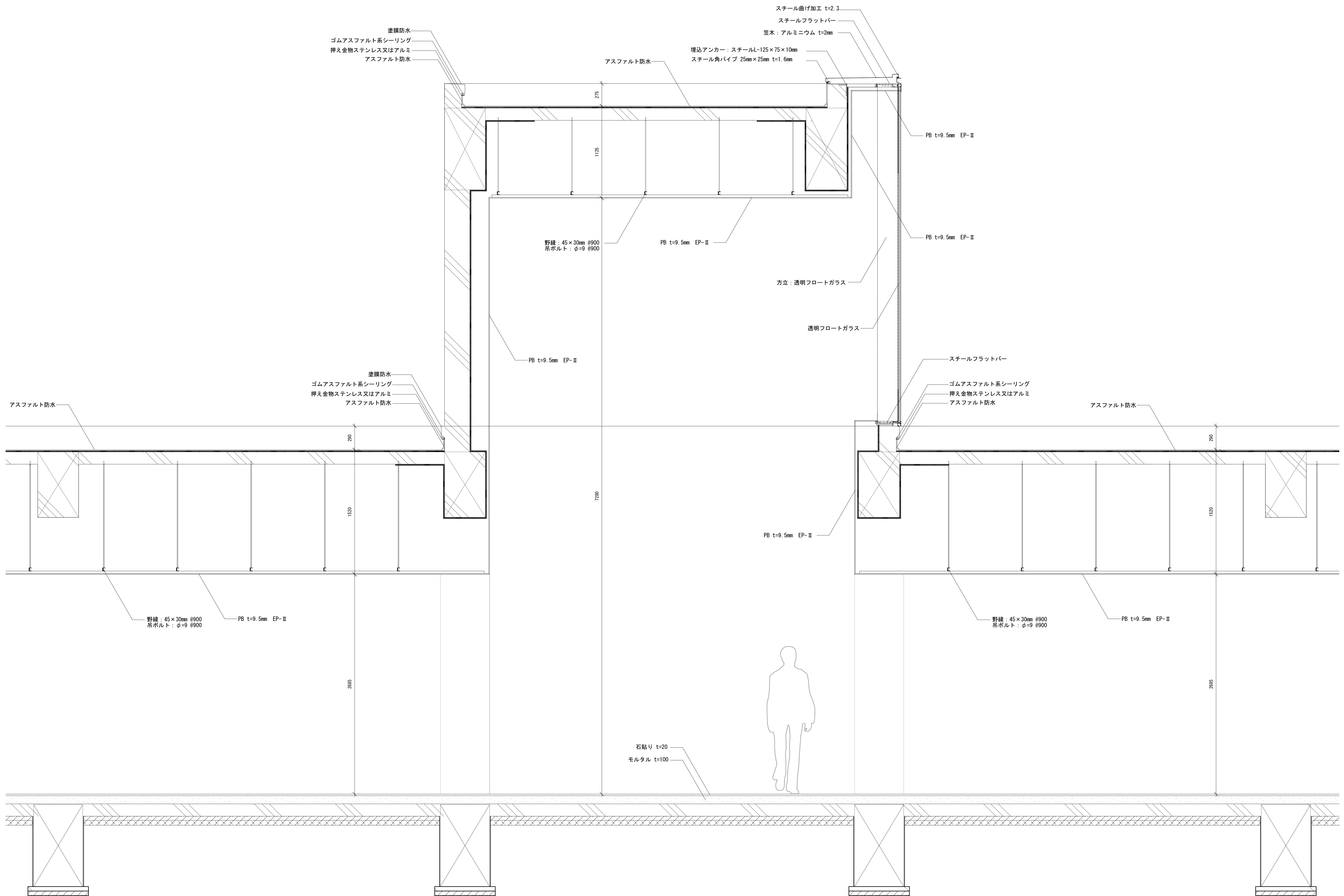
B-B' section
